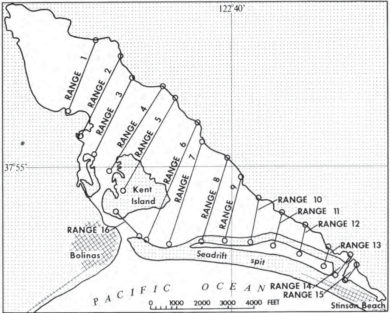
Figure 18a.. USACE Bathymetry Range Lines 1939 (Ritter, 1973).
