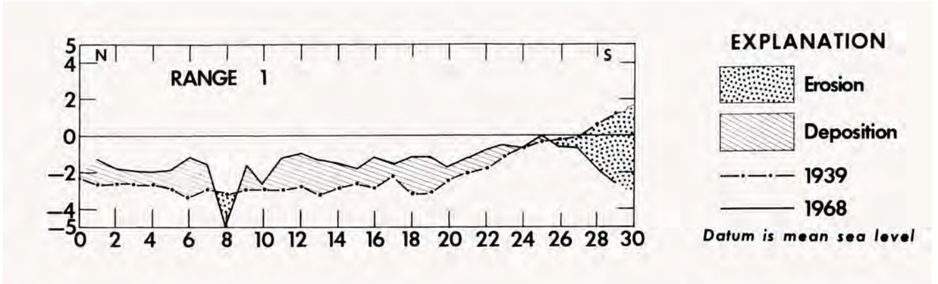
Figure 18b. USACE 1939 and 1968 Range 1 Profiles (Ritter, 1973).
