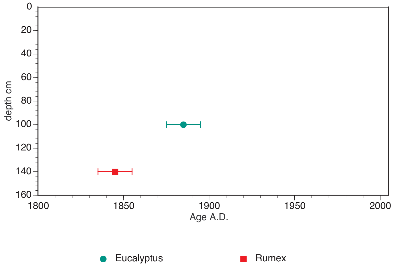
Figure 5a. Age-Depth Curve Core A3
