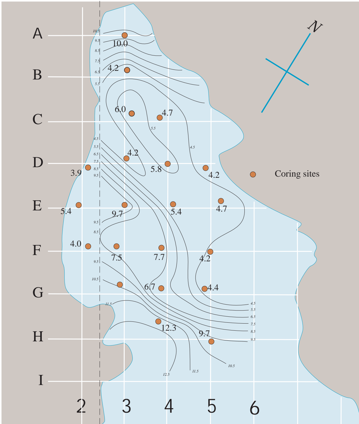
Figure 10. North Basin Sedimentation Rates (mm/year) 1850-1906.
