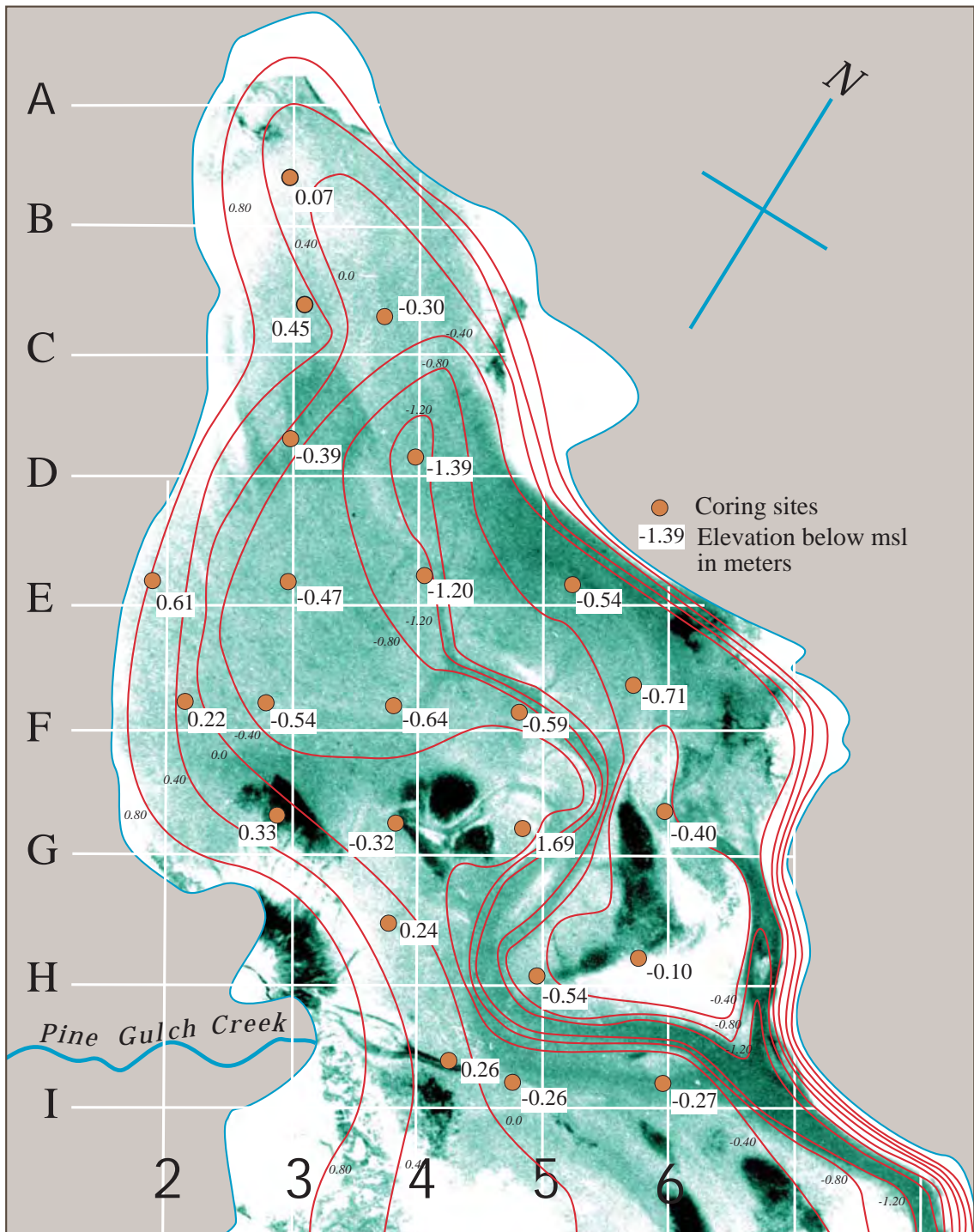
Figure 19. North Basin 2004 Bathymetry with a 1998 USGS Aerial Photograph in the background.
