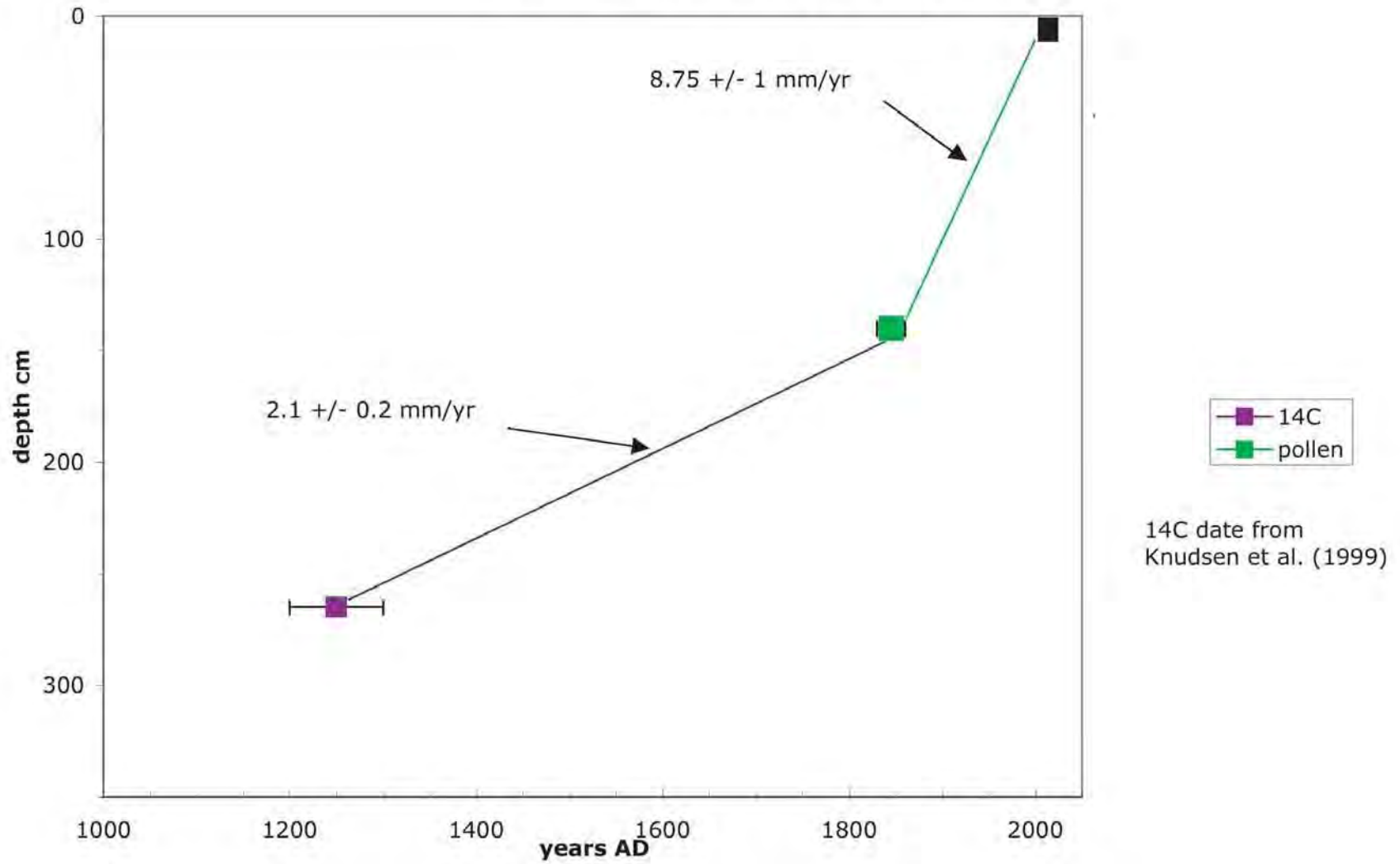
Figure 25b. L2 Age-Depth.
