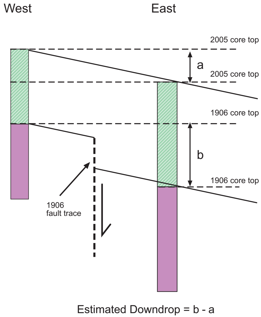
Figure 12. Method of Estimating 1906 Downdrop.
