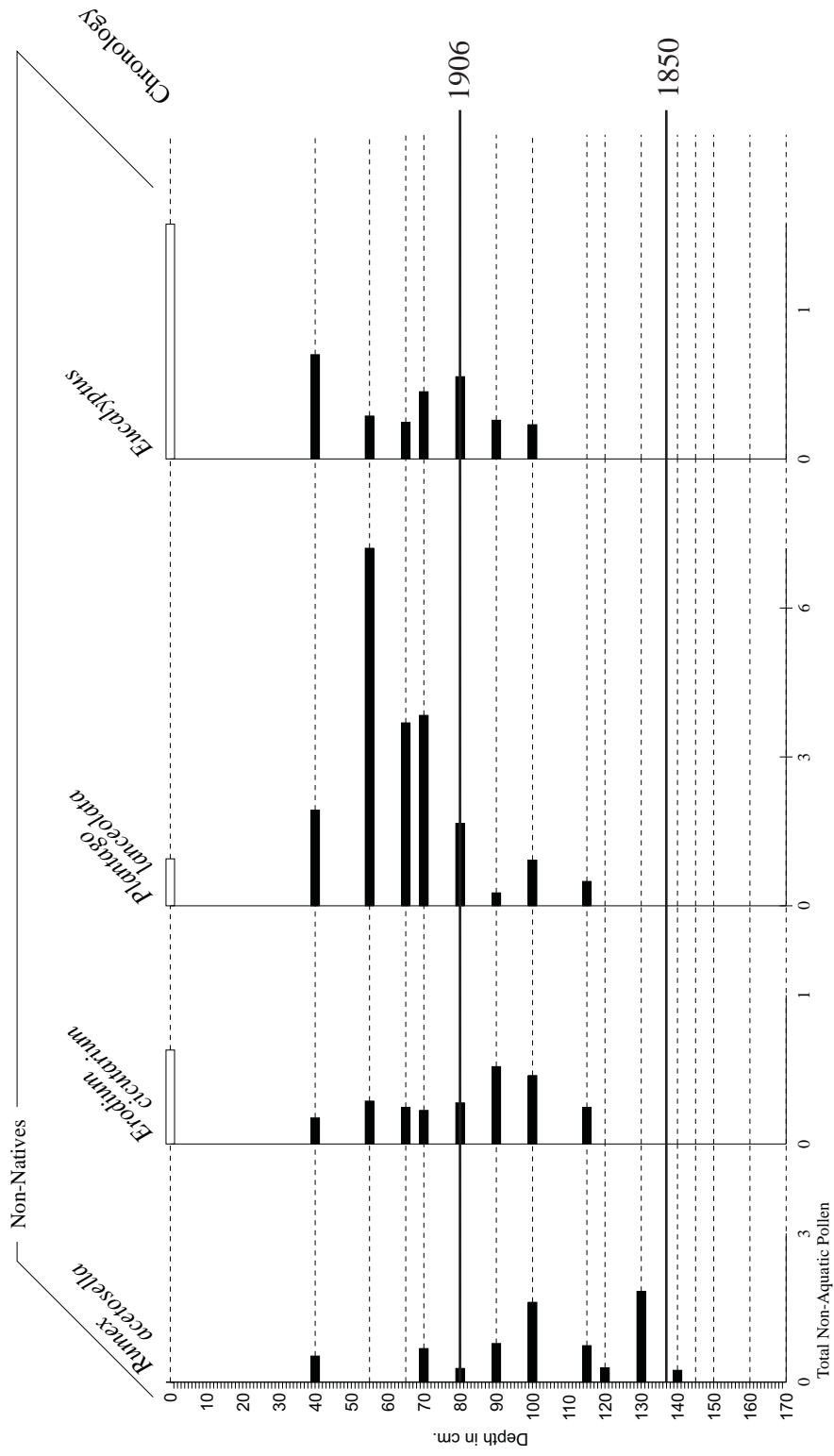
Figure 3a. First Appearance of non-native pollen types and approximate location of 1850 and 1906 horizons in A3.
