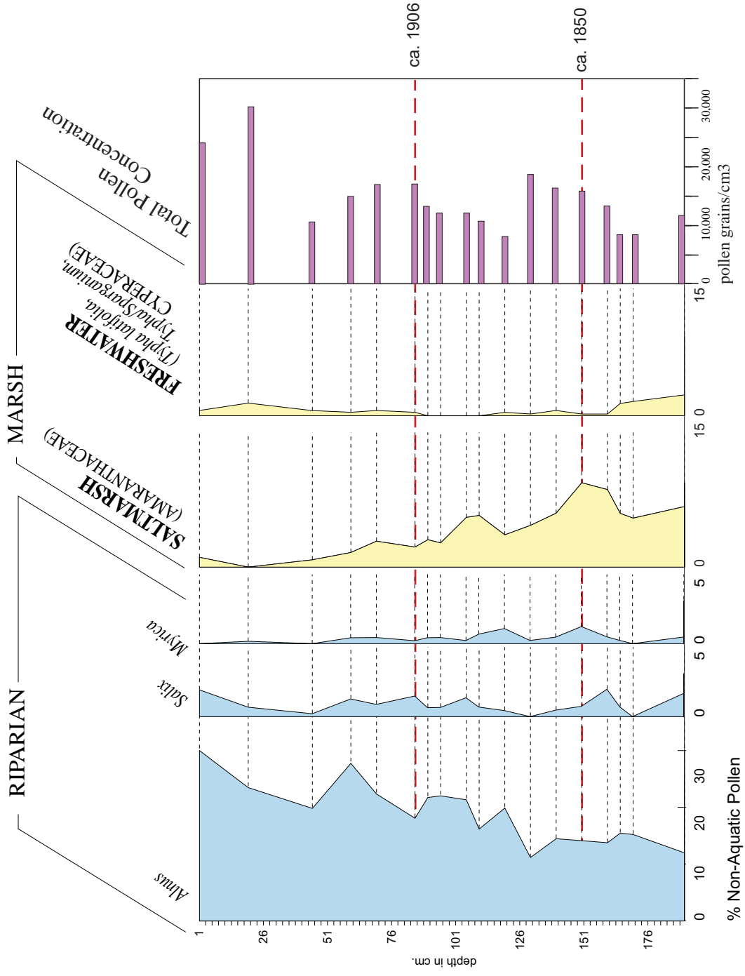
Figure 15d. Core H4 Marsh and Riparian Pollen.
