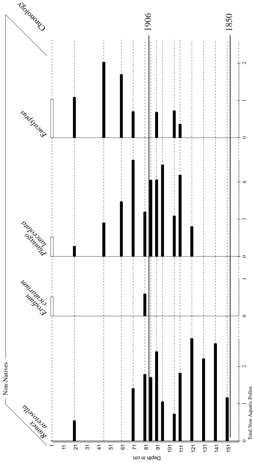
Figure 3d. First Appearance of non-native pollen types and approximate location of 1850 and 1906 horizons in H4.
