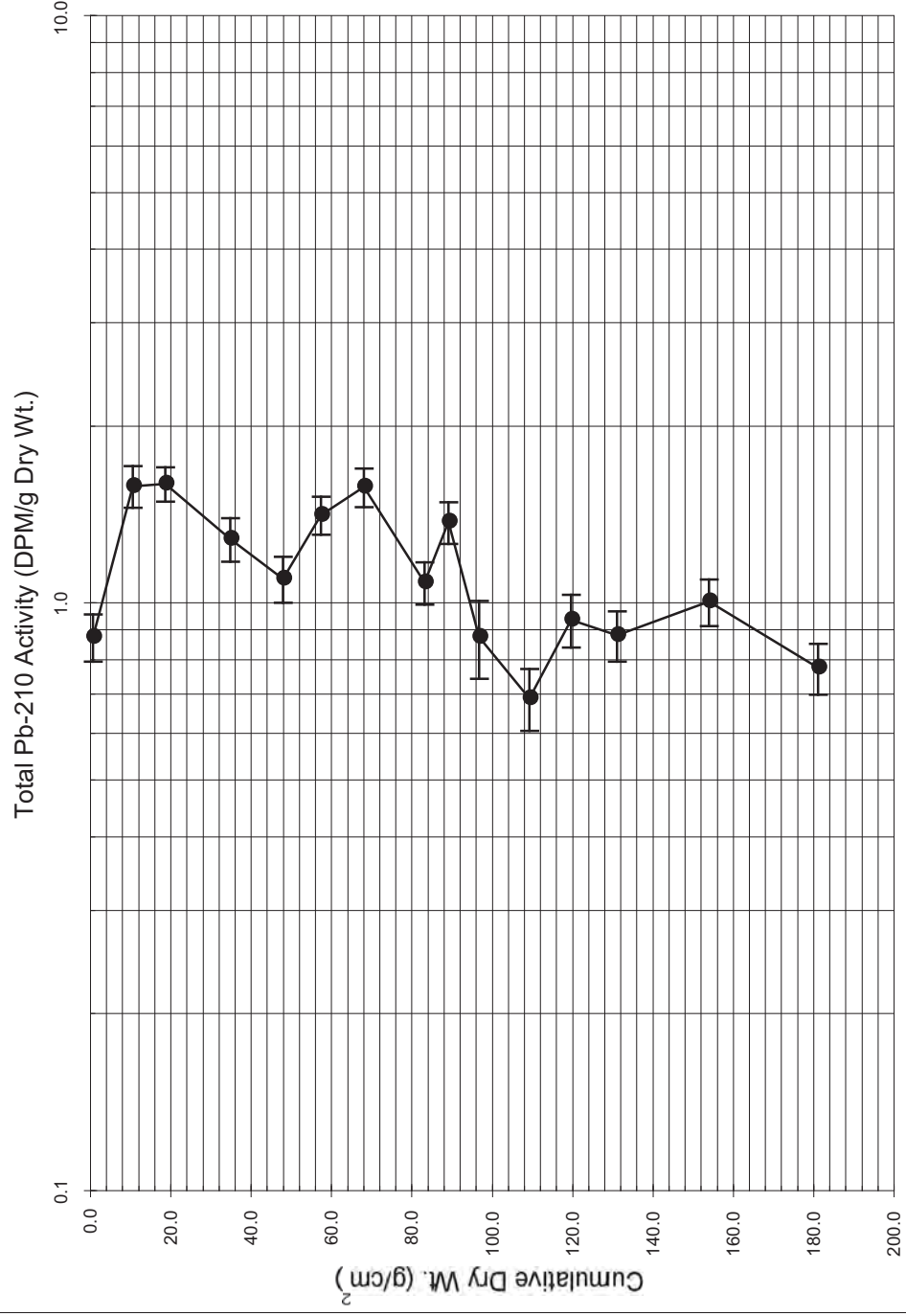
Figure 4a. Total Pb-210 Activity Core C3
