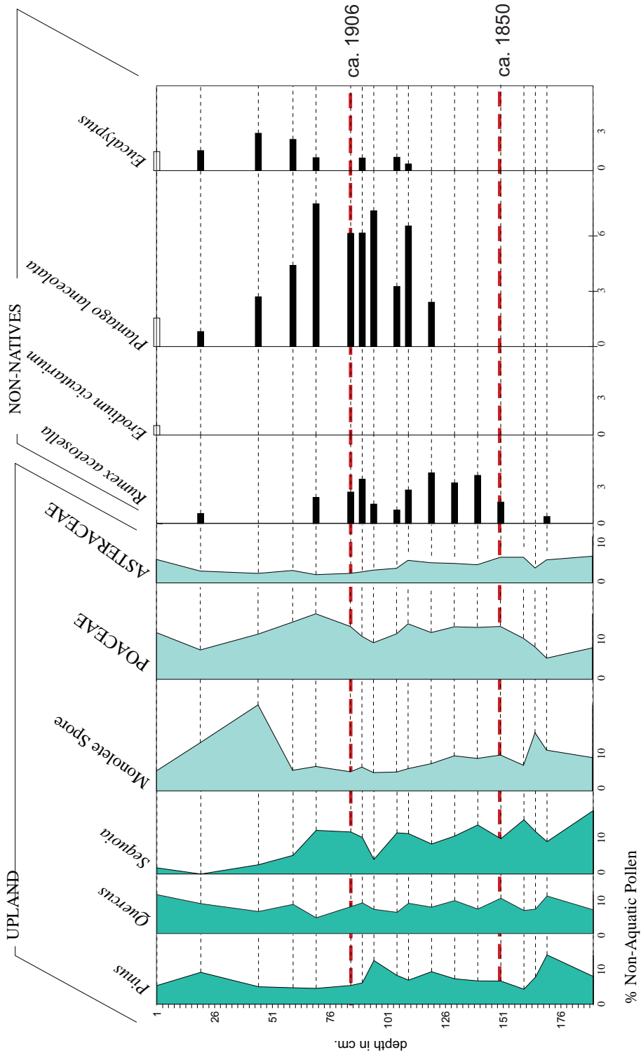
Figure 15c. Core H4 Upland Pollen.
