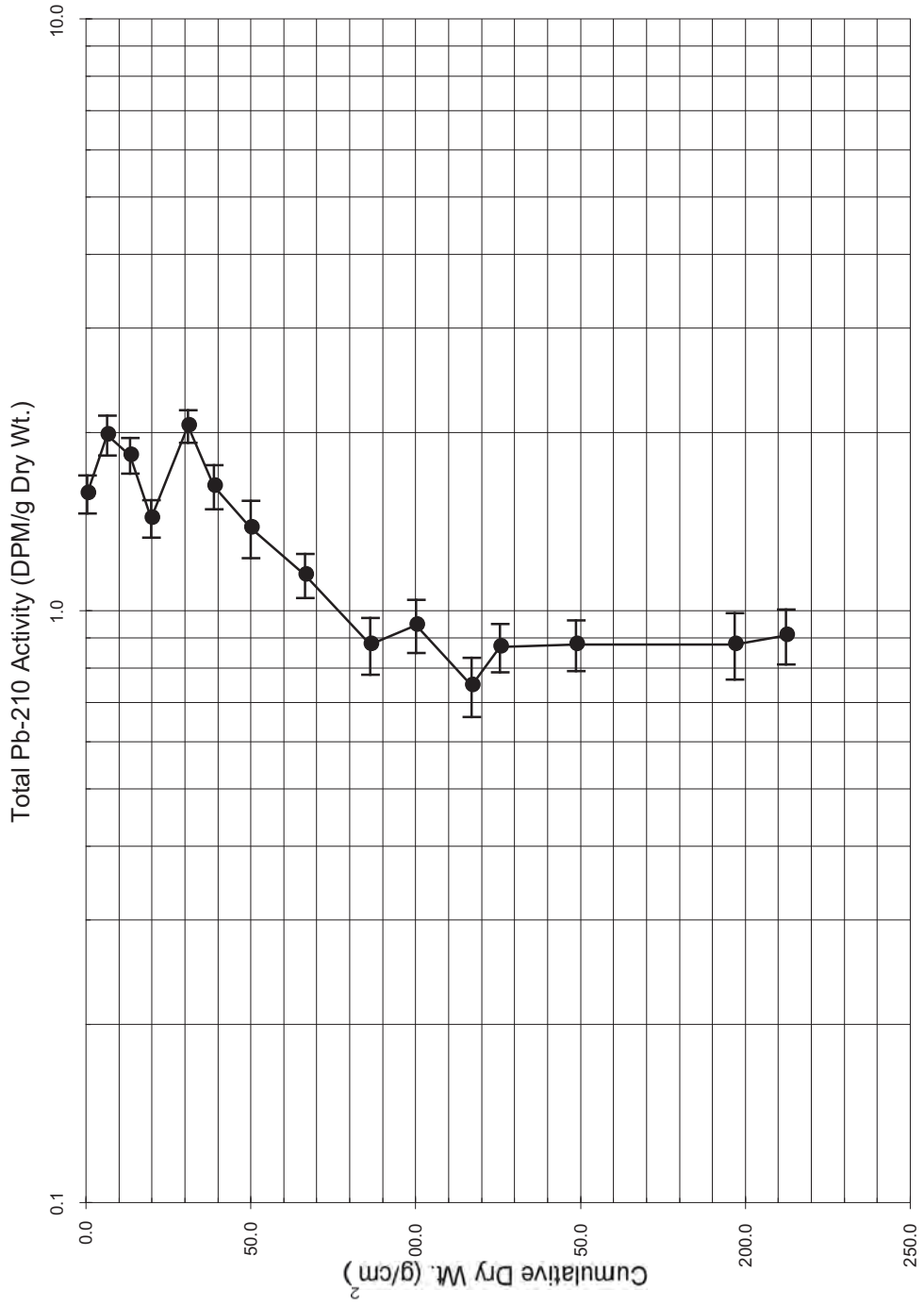
Figure 4b. Total Pb-210 Activity Core H4.
